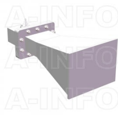
LB-340-10-C-SFSPO Standard Gain Horn Antenna 2.2-3.3GHz 10dB Gain SMA Female
